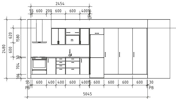
KÖK - K2 SPV ELEVATION A
